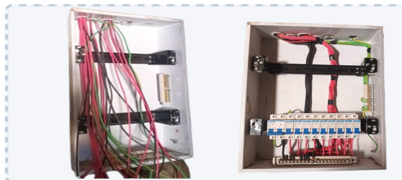
ELECTRICAL DESIGN
